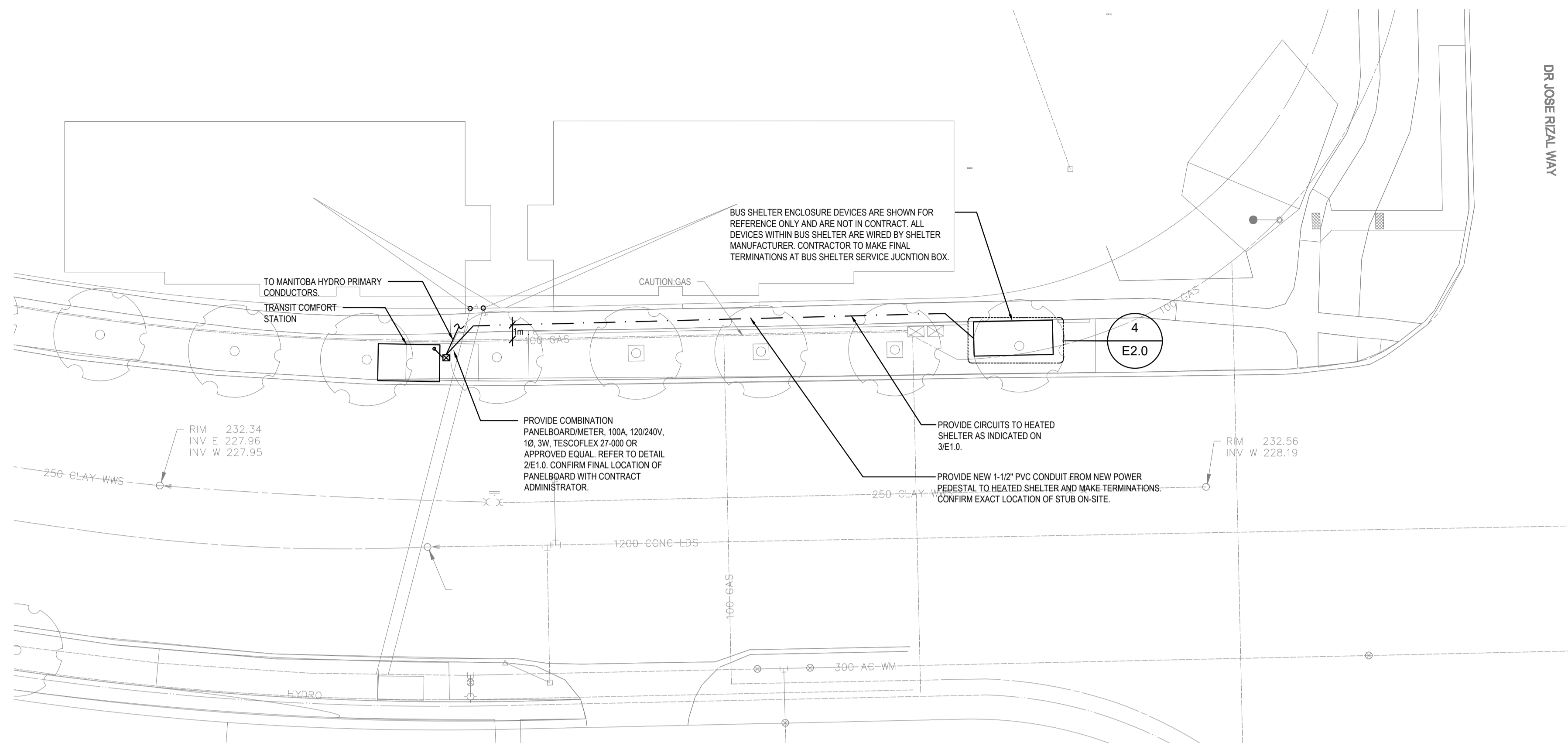
1 OLD COMMONWEALTH - ELECTRICAL SITE PLAN Scale: 1:250
